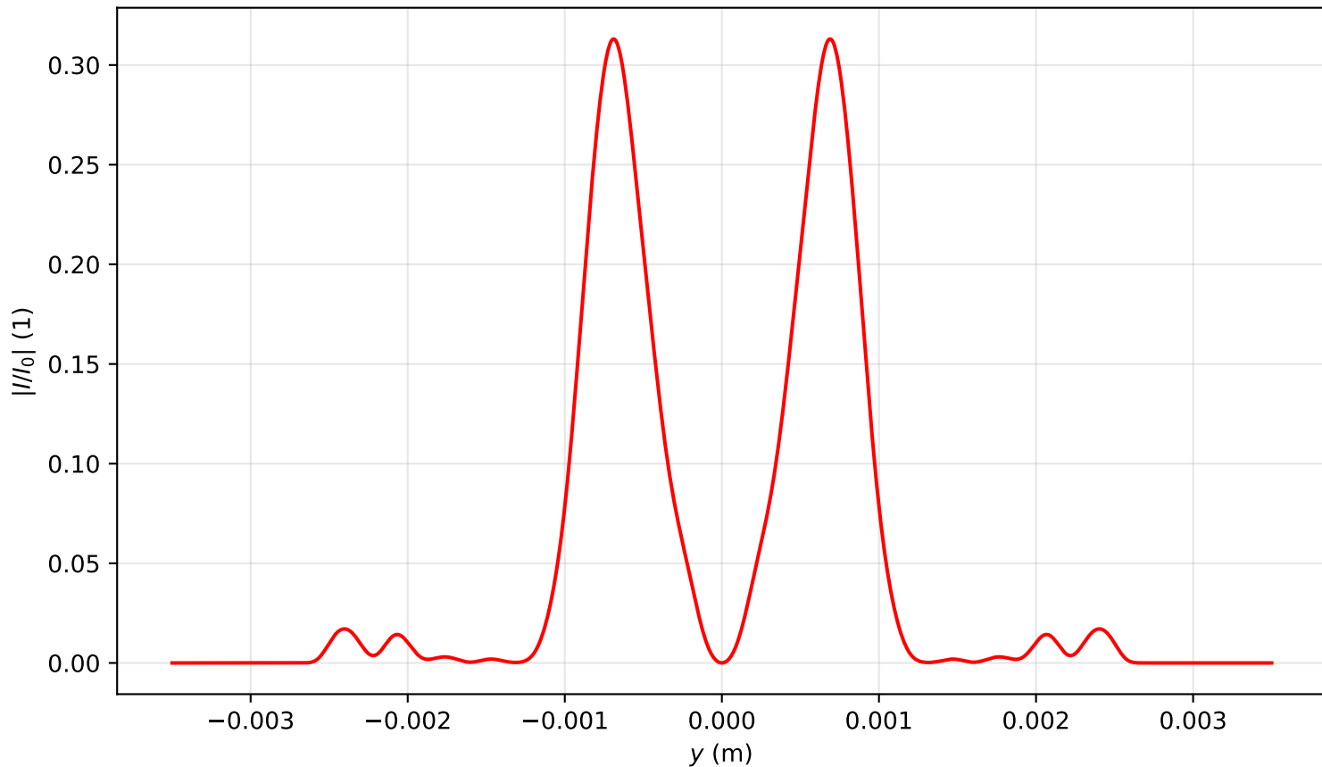
Intensity profile I(x=0, y, z=2.388)/I_0 , P_{in}=7.0P_{cr} , artificial time
